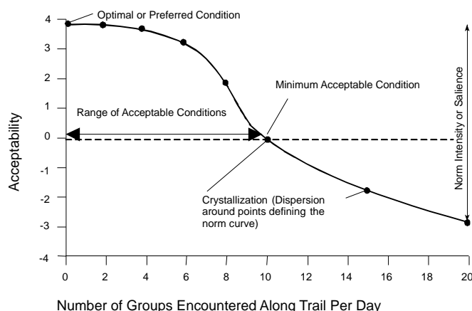
Figure 2—Norm curve.
